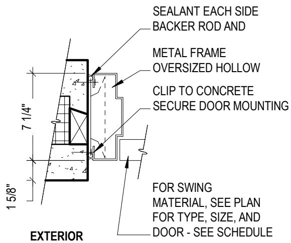
X DX.X DETAIL 1 1/2" = 1'-0"
